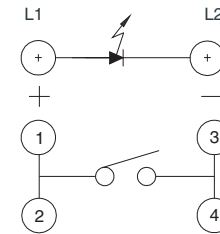
CIRCUIT
