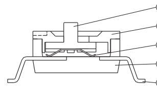
CONSTRUCTION
