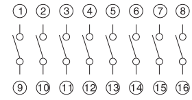
CIRCUIT
