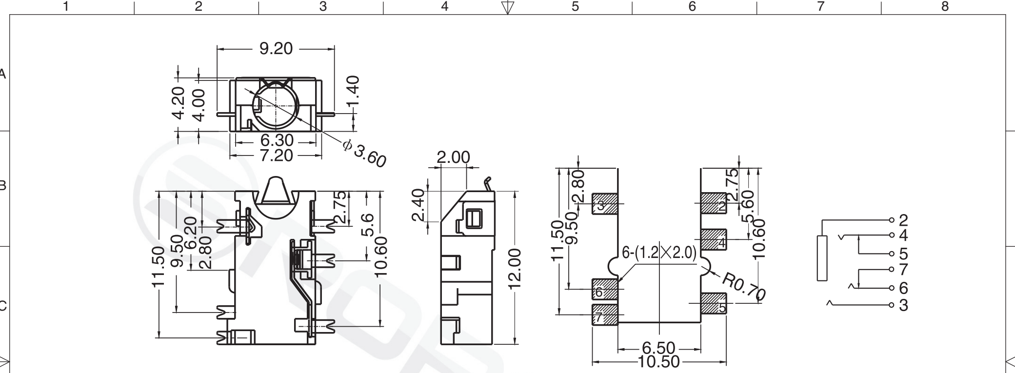
P.C.B LAYOUT TOP VIEW
