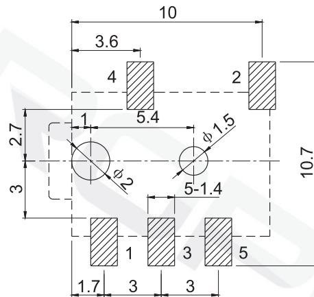
P.C.B Layout(copper-sided view)
