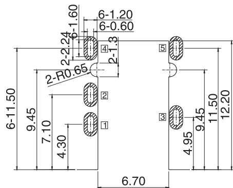
φ 3.50mm 4 POLE PLUG DETAIL DRAWING(1:)
