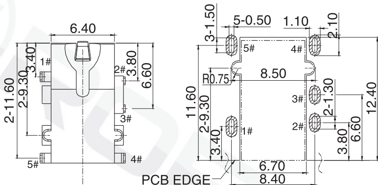
RECOMMEND PCB LAYOUT(TOP VIEW) TOLERANCE: ±0.05
