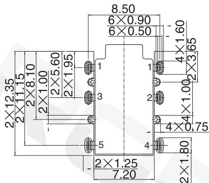
PCB LAYOUT TOP VIEW TOLERANCE: ±0.05
