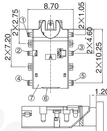
PLUG MATE DRAWING
