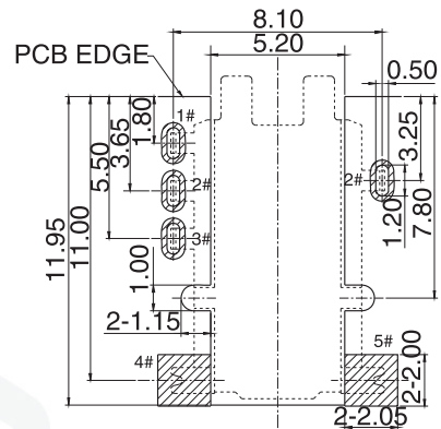
RECOMMEND PCB LAYOUT(TOP VIEW) TOLERANCE:±0.05
