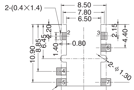
4-(1.9×1.4) P.C.B LAYOUT TOP VIEW
