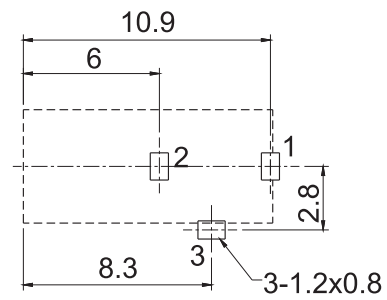
P.C.B Layout(copper-sided view)
