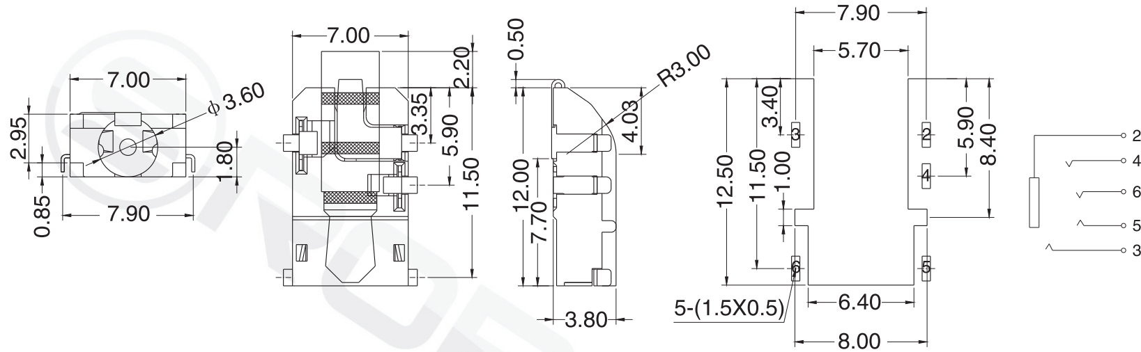
P.C.B LAYOUT TOP VIEW
