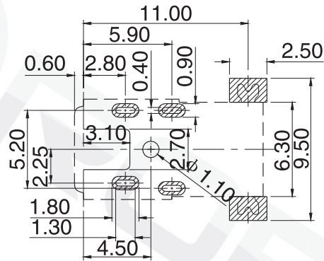
RECOMMENDED PCB LAYOUT TOP VIEW TOL: ±0.05
