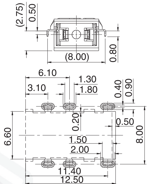
RECOMMENDED PCB LAYOUT TOP VIEW TOL: ±0.05
