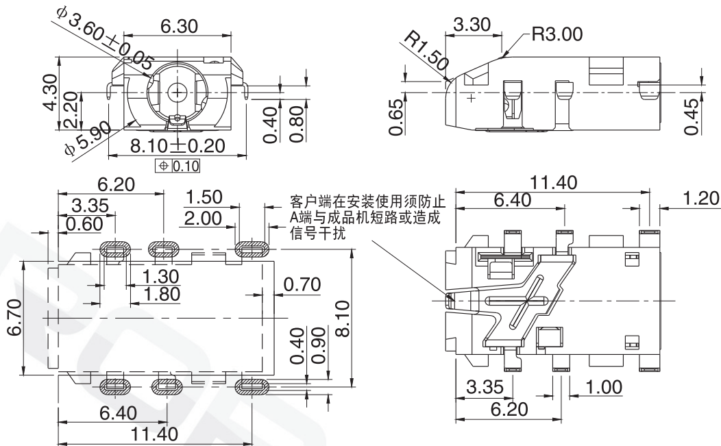
RECOMMENDED PCB LAYOUT TOP VIEW TOL:±0.05
