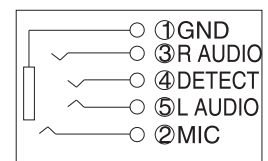
SCHMATIC
