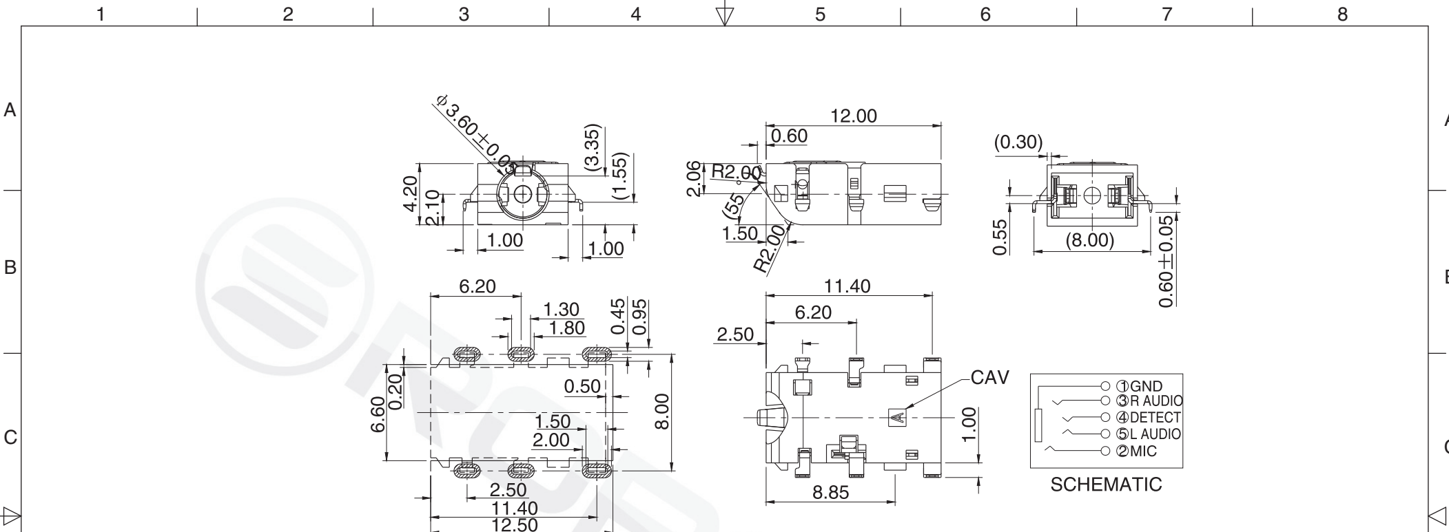
RECOMMENDED PCB LAYOUT TOP VIEW TOL: \pm 0.05
