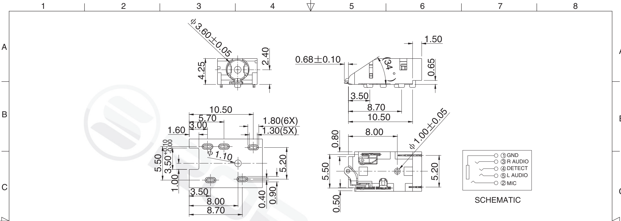
RECOMMENDED PCB LAYOUT TOP VIEW TOL: ±0.05
