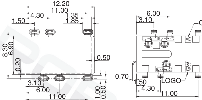
RECOMMENDED PCB LAYOUT TOP VIEW TOL: \pm 0.05
