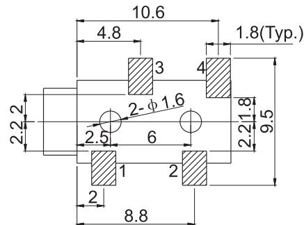
P.C.B Layout(copper-sided view)
