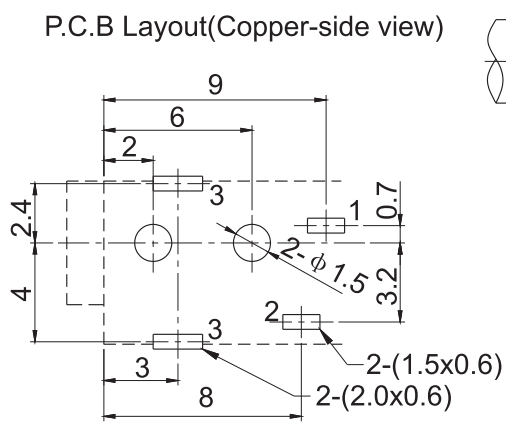
DC MATE PLUG
