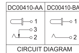
DC MATE PLUG
