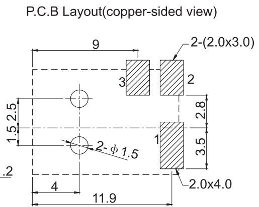
DC MATE PLUG
