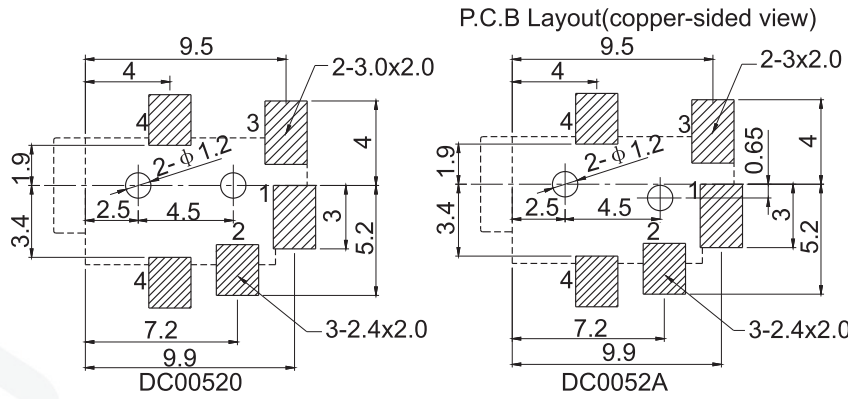
DC MATE PLUG
