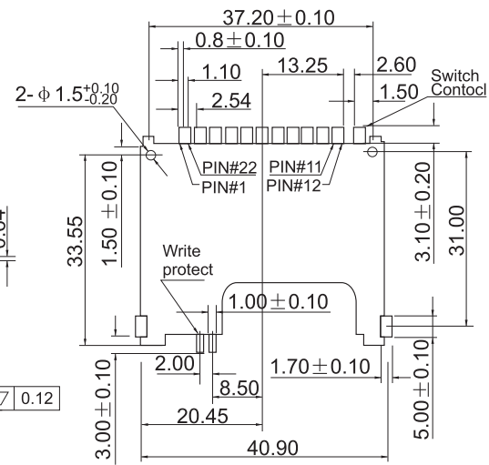
PCB LAYOUT
