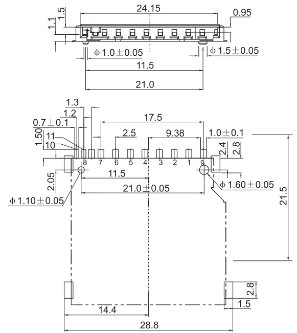
PCB LAYOUT
