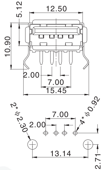
PCB LAYOUT
