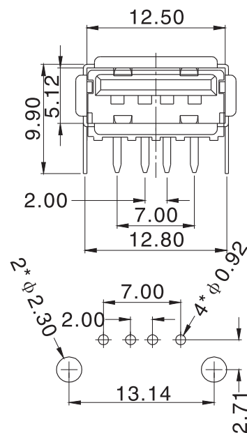
PCB LAYOUT
