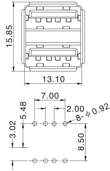
PCB LAYOUT
